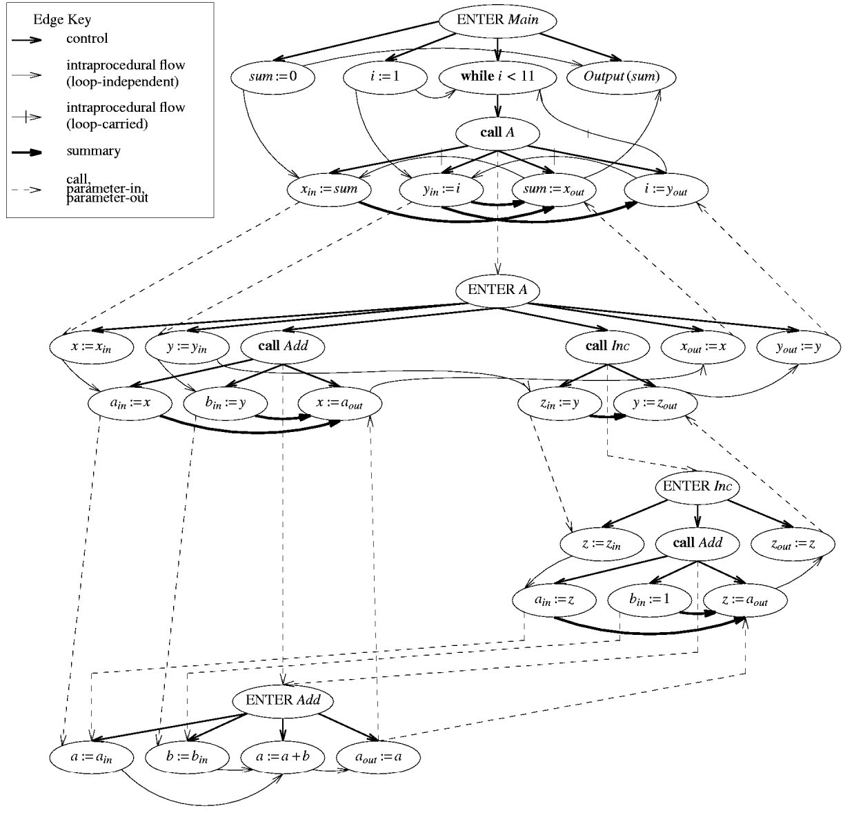
Figure 8: Example system and its SDG.
