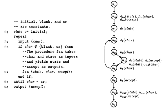
Fig. 3. Module M_2 and its control flow graph G(M_2) .
