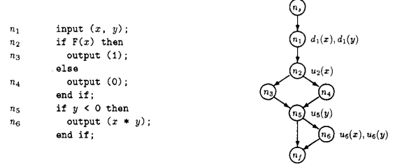
Fig. 9. Module M_7 and its control flow graph G(M_7) .
