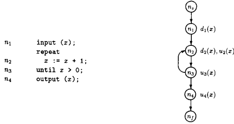
Fig. 4. Module M_3 and its control flow graph G(M_3) .
