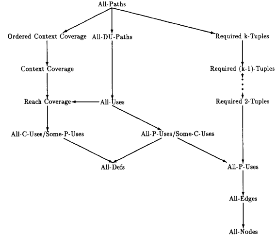
Fig. 8. The new subsumption hierarchy.
