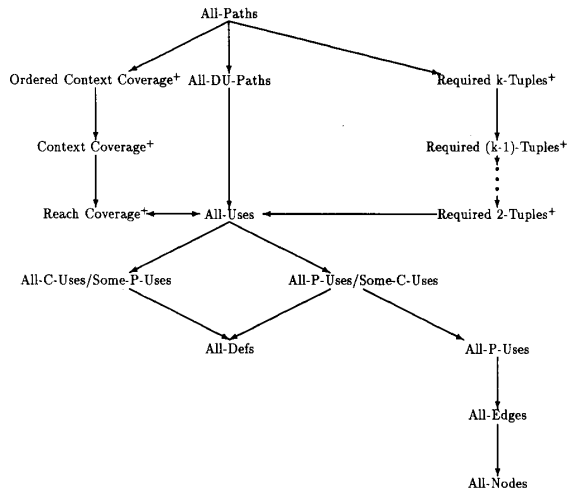
Fig. 10. The final subsumption hierarchy.
