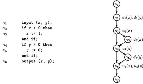
Fig. 2. Module M_1 and its control flow graph G(M_1) .
