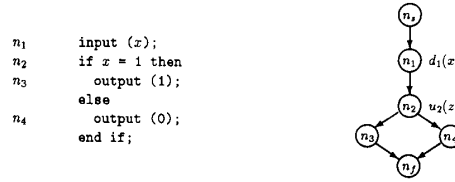
Fig. 6. Module M_5 and its control flow graph G(M_5) .
