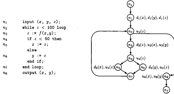
Fig. 5. Module M_4 and its control flow graph G(M_4) .
