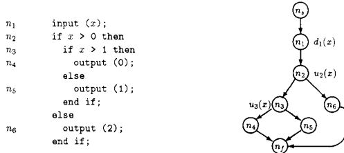
Fig. 7. Module M_6 and its control flow graph G(M_6) .
