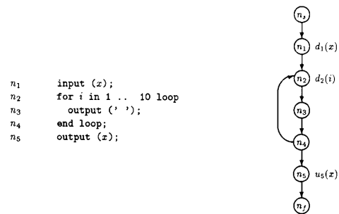
Fig. 11. Module M_8 and its control flow graph G(M_8) .
