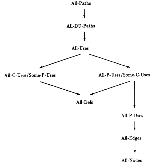
Fig. 1. The Rapps and Weyuker subsumption hierarchy.
