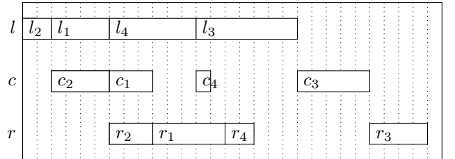
Fig. 5. A Gantt chart of the schedule produced by the PAA algorithm
