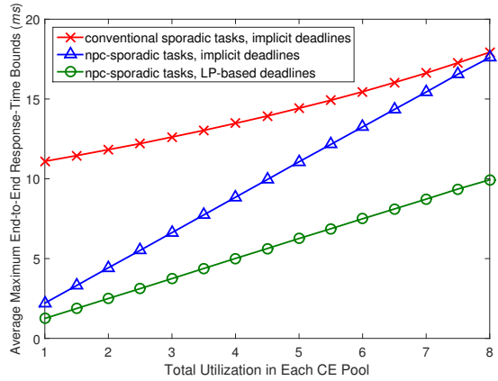
Figure 21: AMERBs as a function of total utilization in each CE pool in the case where each task set has ten DAGs, 20 tasks per DAG, and \text{edgeProb}=0.2 .
