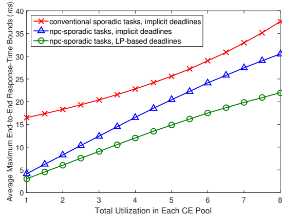
Figure 16: AMERBs as a function of total utilization in each CE pool in the case where each task set has five DAGs, 20 tasks per DAG, and \text{edgeProb}=0.5 .
