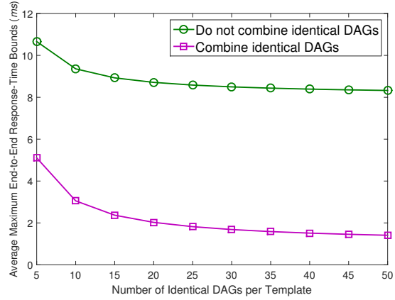
Figure 40: AMERBs as a function of the number of identical DAGs per template in the case where total utilization in each CE pool is fixed to eight, each task set has five templates, each DAG has 20 tasks, and edgeProb=0.5.
