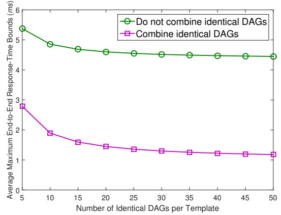
Figure 45: AMERBs as a function of the number of identical DAGs per template in the case where total utilization in each CE pool is fixed to eight, each task set has ten templates, each DAG has 20 tasks, and edgeProb=0.2.
