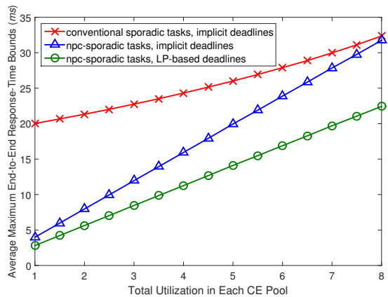
Figure 23: AMERBs as a function of total utilization in each CE pool in the case where each task set has ten DAGs, 20 tasks per DAG, and \text{edgeProb}=0.8 .
