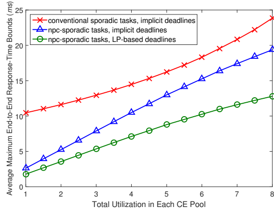
Figure 15: AMERBs as a function of total utilization in each CE pool in the case where each task set has five DAGs, 20 tasks per DAG, and \text{edgeProb}=0.2 .
