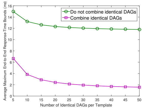
Figure 41: AMERBs as a function of the number of identical DAGs per template in the case where total utilization in each CE pool is fixed to eight, each task set has five templates, each DAG has 20 tasks, and edgeProb=0.8.
